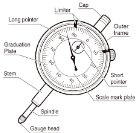
Fig: Dial Indicator
